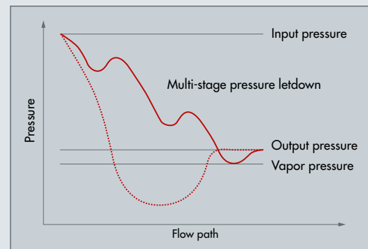
Pressure graph: — With AC-trim ..... Without AC-trim
