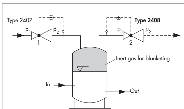
Fig. 2 · Functional diagram of Type 2408
