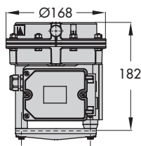
Type 3372/120 cm 2 with Type 3725 fail-close and fail-open
