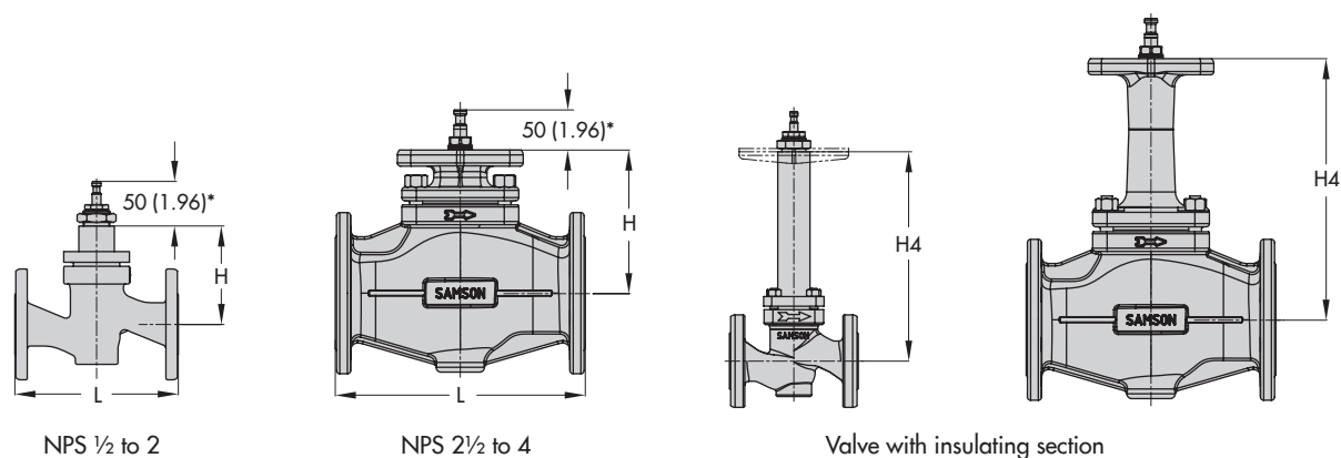
Dimensional drawings for Type 3321 Valve
