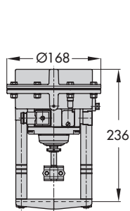
Type 3372/120 cm 2 integrated, fail-close
