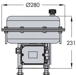
Type 3372/350 cm 2 with Type 3725 fail-close and fail-open
