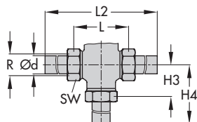
Version with male thread connection and welding ends
